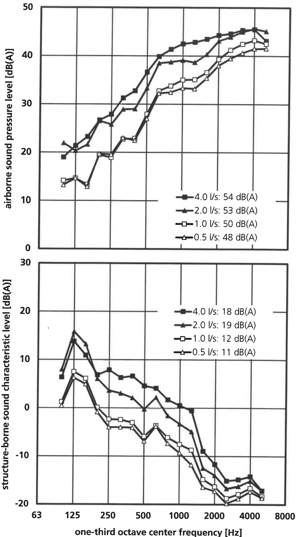
Frequency spectrum of the airborne sound pressure level L_{a,A} (above) and structure-borne sound characteristic level L_{sc,A} (below) measured at various flow rates according to EN 14366.
